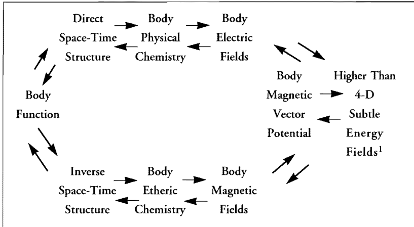
Figure 1. Reaction equation.
